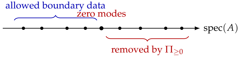
Figure 10: The APS condition is nonlocal: it uses the global spectral decomposition of the tangential operator rather than pointwise boundary values.
